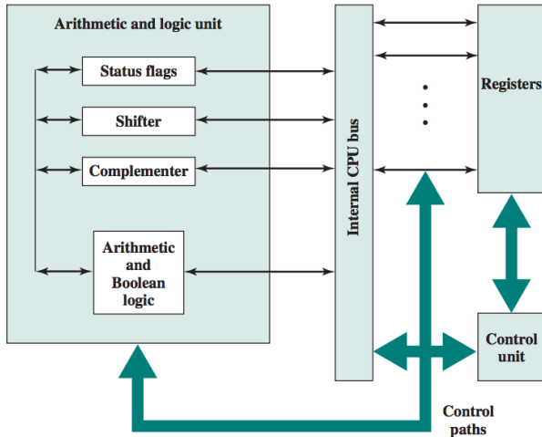
Figure: Internal structure of the CPU(Source: (Stallings, 2015))
