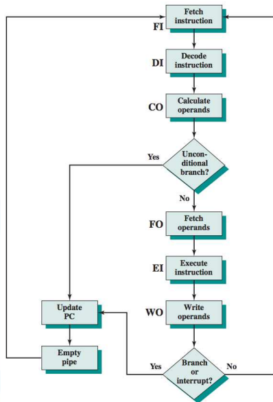
Figure: Six-Stage CPU Instruction Pipeline (Source: (Stallings, 2015))
