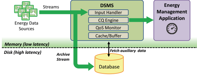
Fig. 3: Data stream processing using a DSMS. Data streams generated from several sources are directly processed by the DSMS, highly decreasing the latency of data processing. Data streams may be persisted (for computation that require past data), without affecting ongoing continuous queries evaluation.
