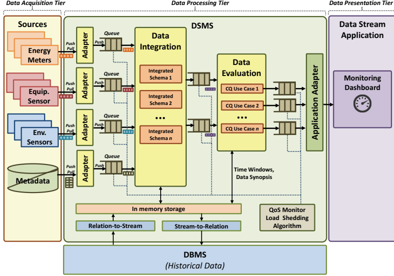
Fig. 5: Proposed Architecture. From left to right: Data Acquisition Tier composed of the data streaming sources. Data Processing Tier responsible for the integration, validation, normalization of gathered data, and, if necessary, persists them for future reference. Data Presentation Tier where produced results will be passed to the stream application.
