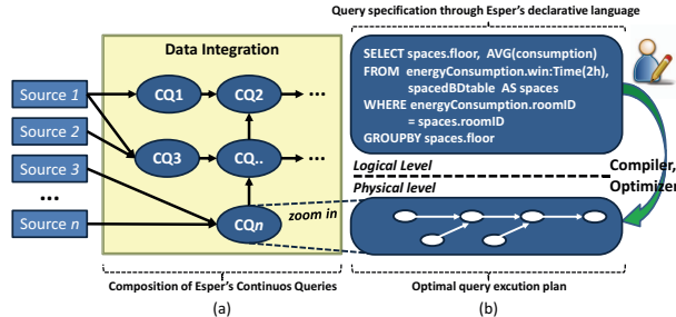
Fig. 6: Data processing as a graph of Continuous Queries (CQs). (a) The data transformation components (e.g. Data Integration) are implemented through a composition of CQs. (b) Each CQ works as a data transformation step (in a pipeline of transformations), and is specified through Esper’s declarative language, to then be transparently compiled to an optimal query execution plan.
