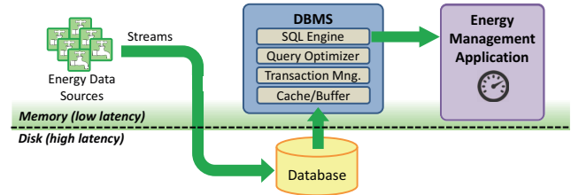
Fig. 2: Data stream processing using a DBMS. Data streams produced by sources are first persisted into a database, and only then processed by the DBMS. For the data stream application this introduced delay is unacceptable.
