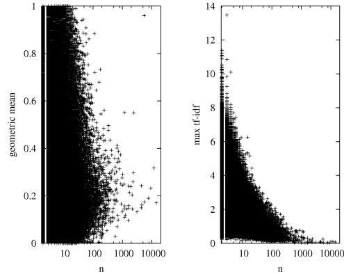
Fig. 1. On left, URL weight contribution geometric mean versus URL coverage size n . On right, given the set of terms associated to the queries covered by each URL, URL maximum tf-idf score versus URL coverage size n .
