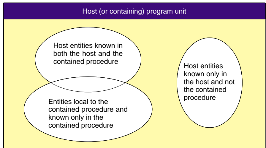
Figure 18. Host association
