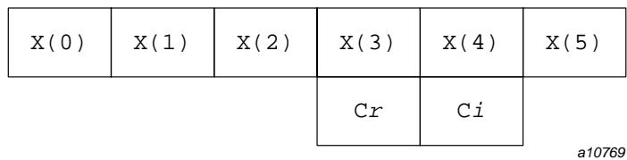
Figure 21. Example 1
