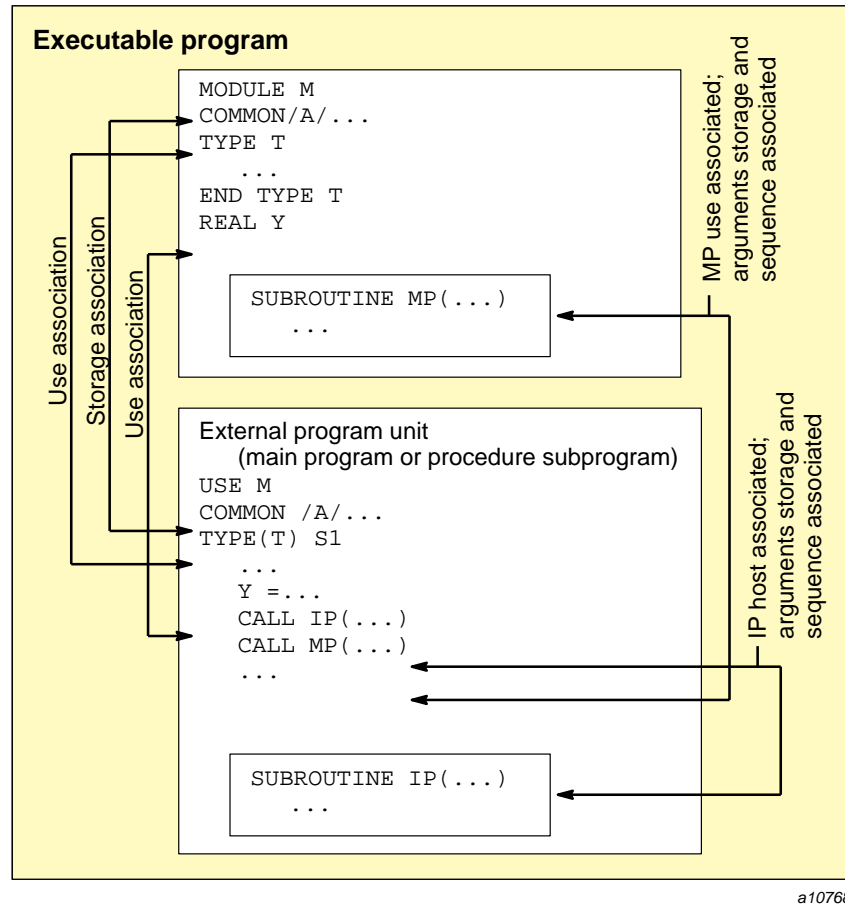
Figure 17. Associations between a module scoping unit and a nonmodule scoping unit
