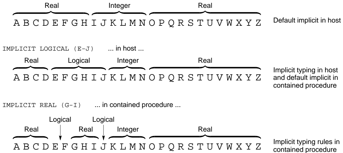
Figure 20. How the mapping of implicit typing progresses from host to contained procedure
