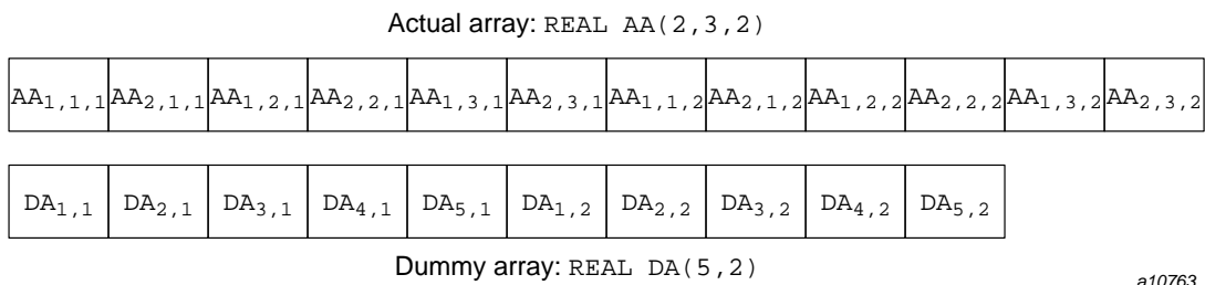
Figure 12. Example of array element sequence association
