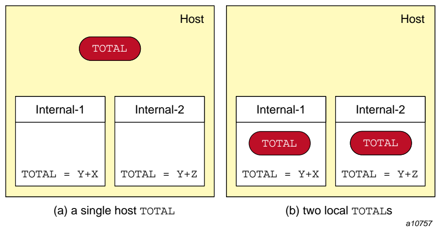
Figure 19. Is there one TOTAL in the host or two local TOTAL s?
