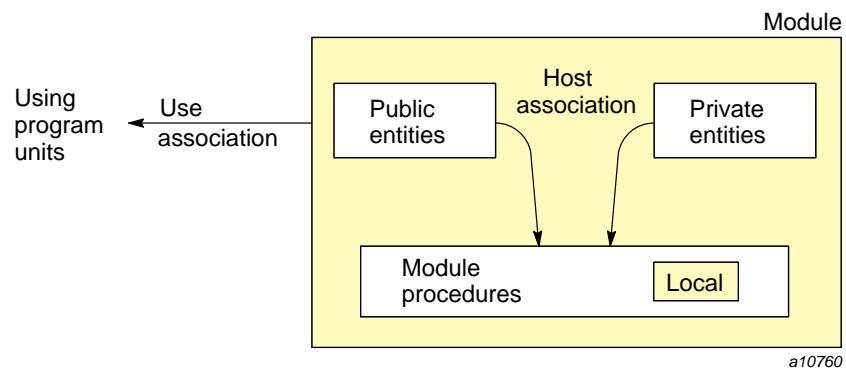
Figure 9. Use of public and private module entities
