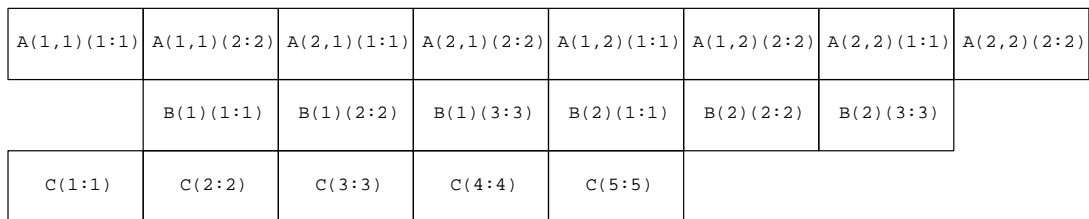
Figure 22. Example 2
