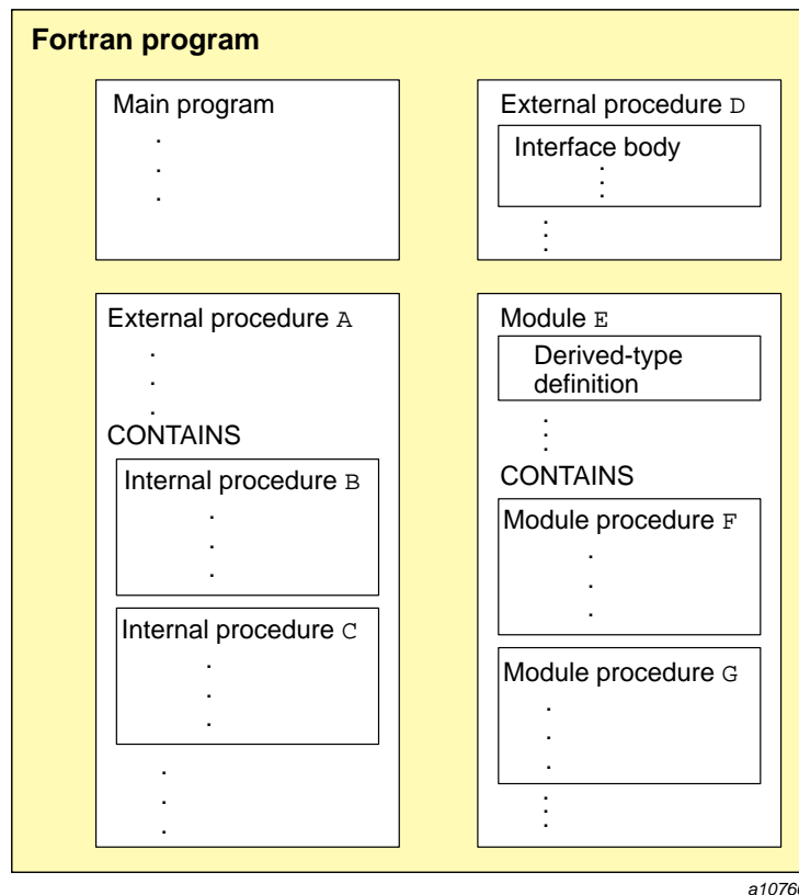
Figure 15. Scoping units
