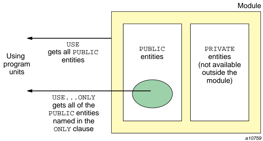
Figure 8. Public and private entities in a module
