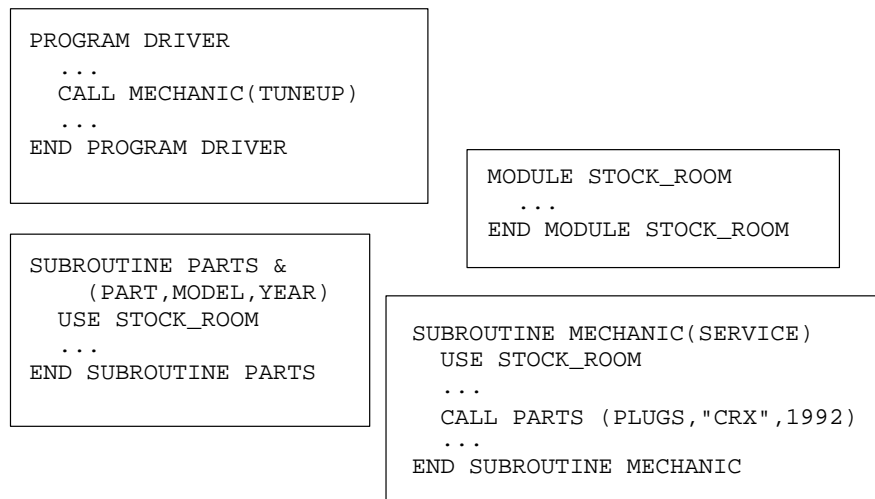
Figure 7. Four program units
