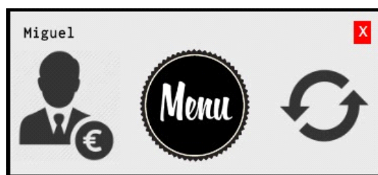
Figura 6: Menu principal
