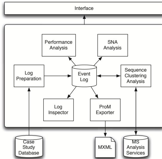
Figure 7: Architecture of the Medtrix Process Mining Studio.
