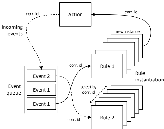
Fig. 9. Rule engine
