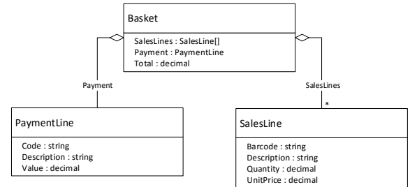
Fig. 4. Data elements for the sales basket (simplified)
