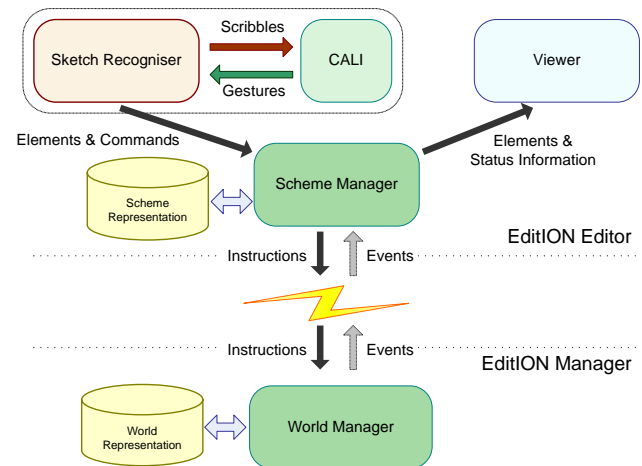
Figure 3. EditION architecture
