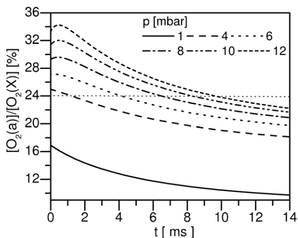
Figure 12. O_2(a) yield as a function of afterglow time at different pressures in the case of 90%Ar–10% O_2 initial mixture composition.
