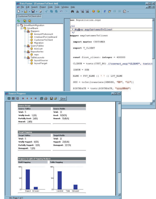
Figure 4: Snapshot of DATA FUSION IDE
