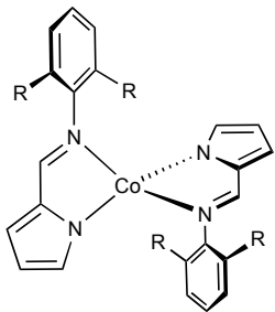
[Co(L1) 2 ] (a)
