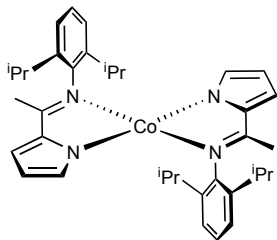
[Co(L1) 2 ] (b)
