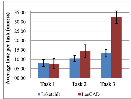
Figure 6: Average time to complete each task.
